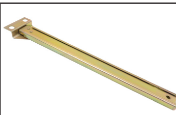
Telescopic Bonnet Lid Stay Open: 490mm/Closed: 285mm
